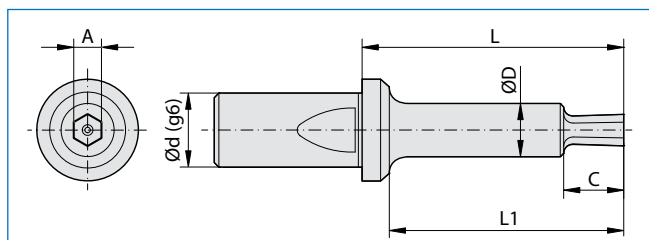
"G16L" - "G16LK" STANDARD "G16L" - "G16LK" STANDARD
