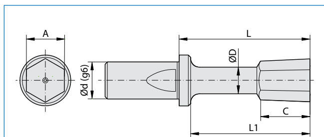
"G16L" - "G16LK" STANDARD "G16L" - "G16LK" STANDARD
