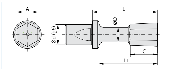
"G16M" - "G16MK" STANDARD "G16M" - "G16MK" STANDARD
