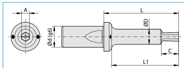
"G16LC" - "G16LKC" CON PASSAGGIO REFRIGERANTE INTERNO "G16LC" - "G16LKC" WITH INTERNAL FLOW OF COOLANT
